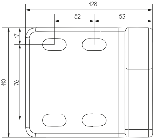
UNIVERSAL BRACKET Wall Ceiling
