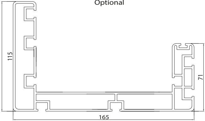
PROFILE FREESTANDING GUTTER Optional
